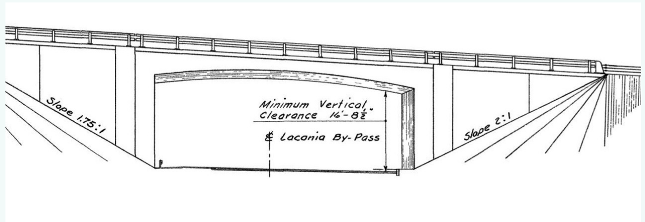
Original drawing of the west elevation, 1963 (NHDOT)
