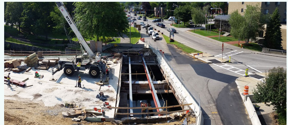
2014 Beacon Street East reconstruction, looking south (Dubois & King)
